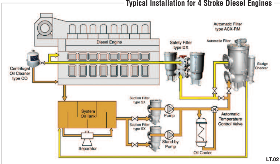
Typical Installation for 4 Stroke Diesel Engines
